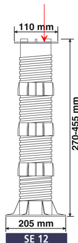
Figure 2 Typical "ETERNO SE12" specimen.
