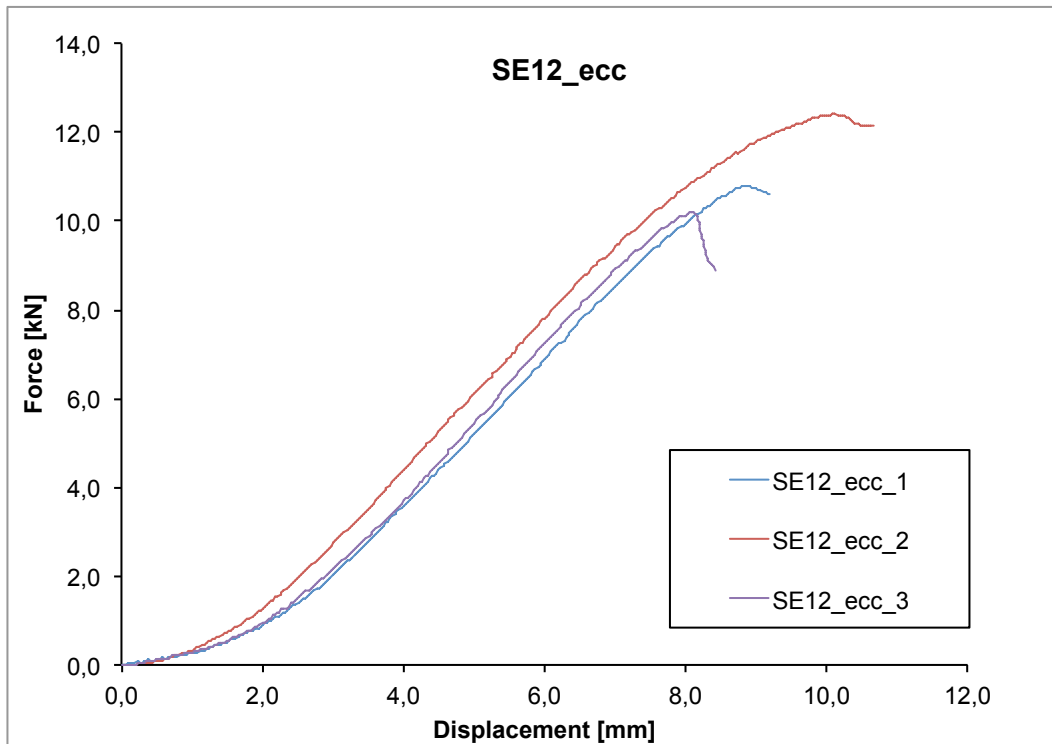
Figure 1 Diagram force versus displacement of testing machine's crossbar for "ETERNO SE12" specimen.
