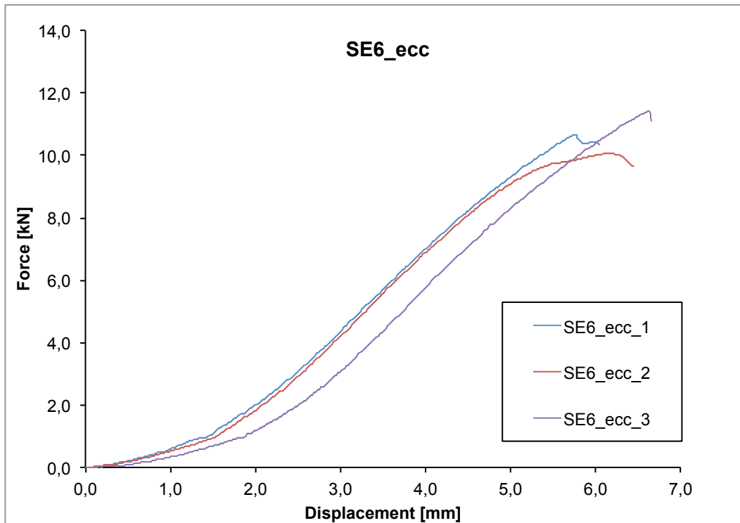
Figure 1 Diagram force versus displacement of testing machine's crossbar for "ETERNO SE6" specimen.
