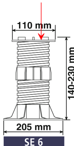
Figure 2 Typical "ETERNO SE6" specimen.
