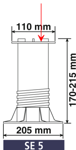
Figure 2 Typical "ETERNO SE5" specimen.
