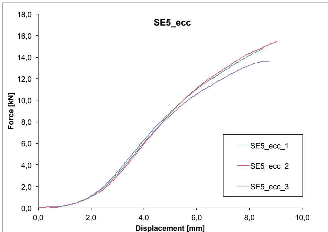
Figure 1 Diagram force versus displacement of testing machine's crossbar for "ETERNO SE5" specimen.
