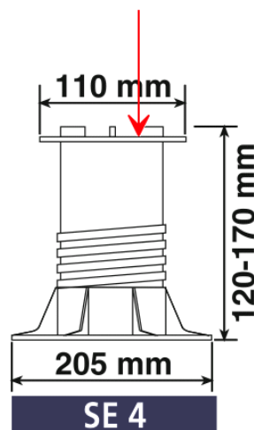
Figure 2 Typical "ETERNO SE4" specimen.
