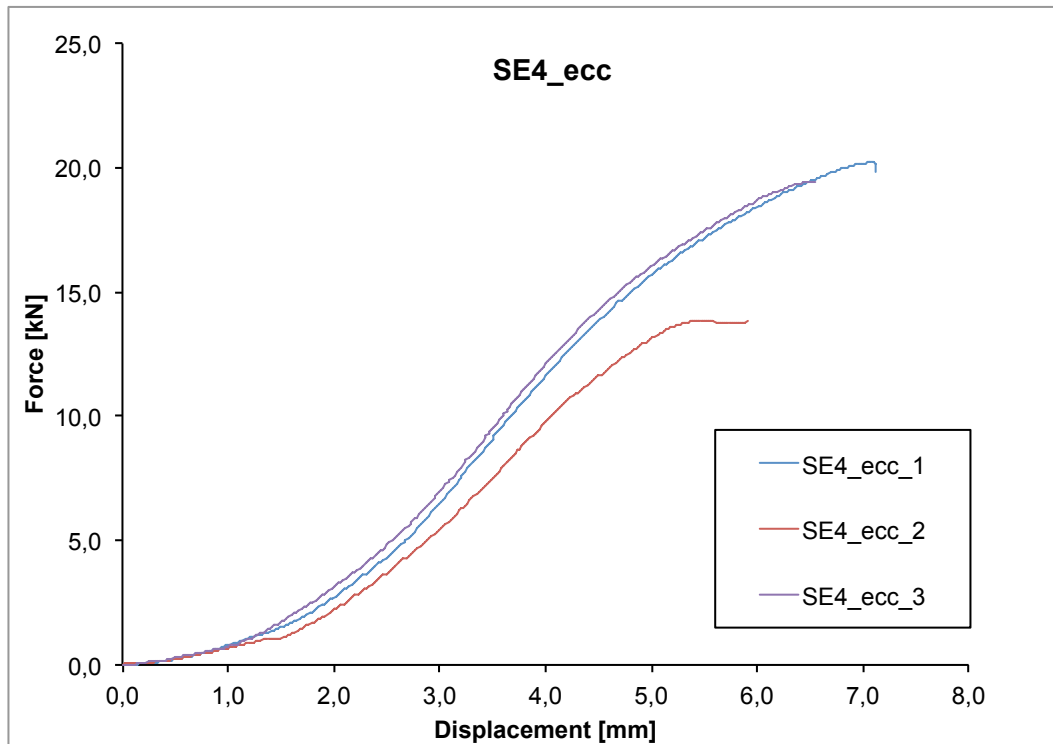
Figure 1 Diagram force versus displacement of testing machine's crossbar for "ETERNO SE4" specimen.
