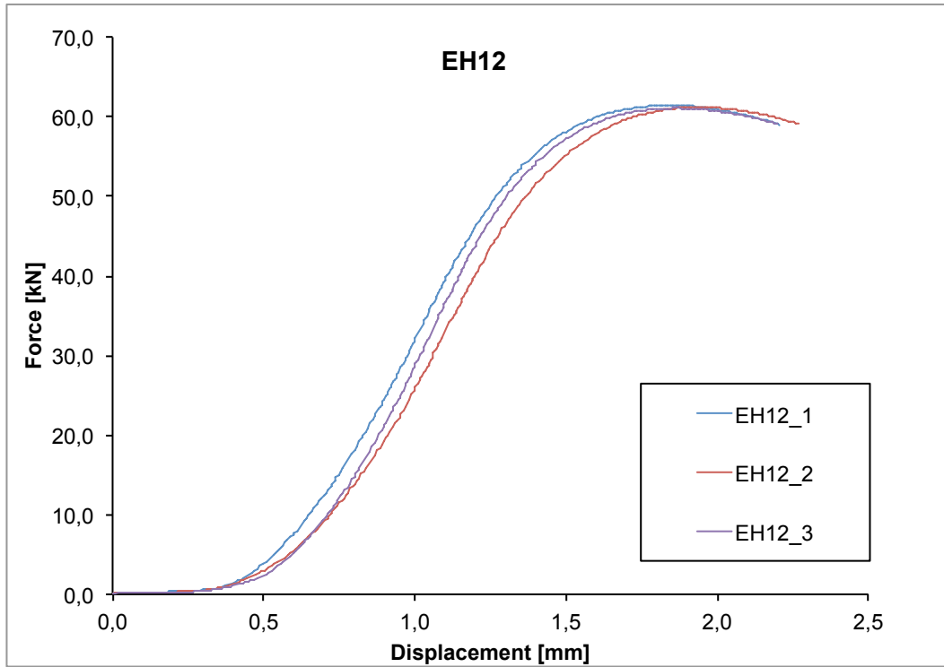
Figure 1 Diagram force versus displacement of testing machine's crossbar for "EH12" support specimen.
