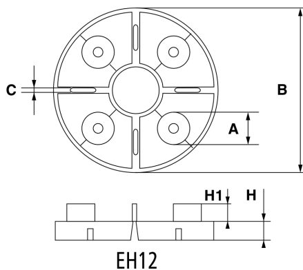
Figure 2 Typical "EH12" support specimen.
